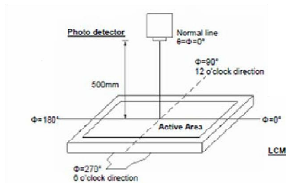
Fig. 6-2 Optical measurement system
